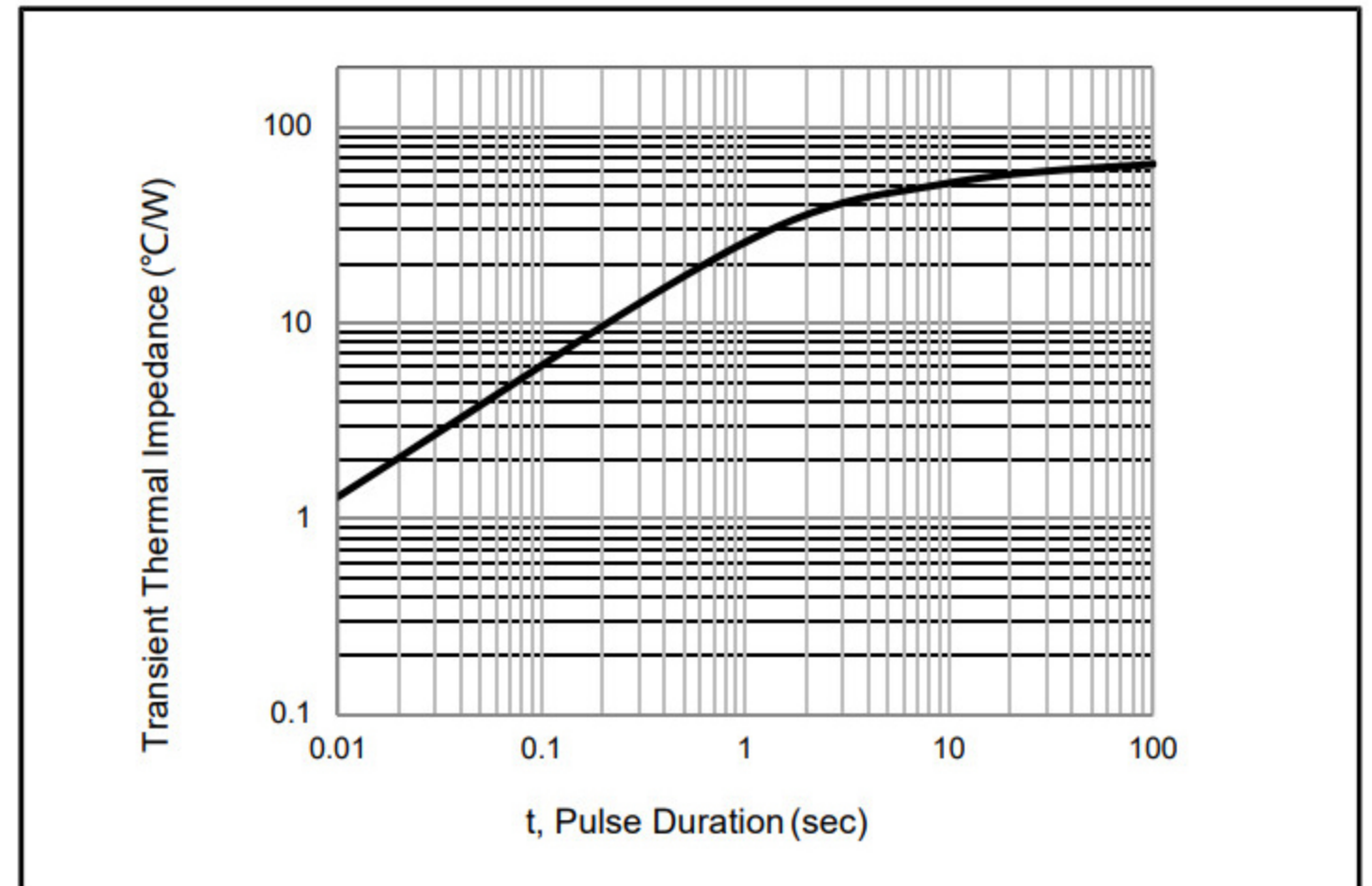
Fig. 6 - Typical Transient Thermal Impedance
