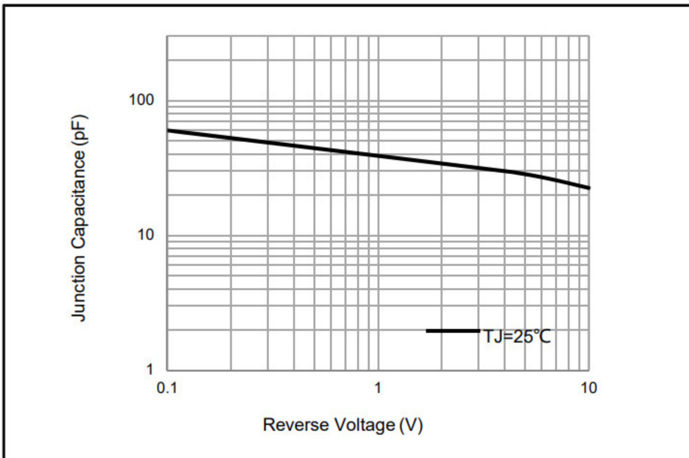
Fig. 5 - Typical Junction Capacitance
